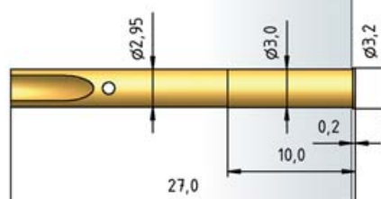
H 1060/G-L
